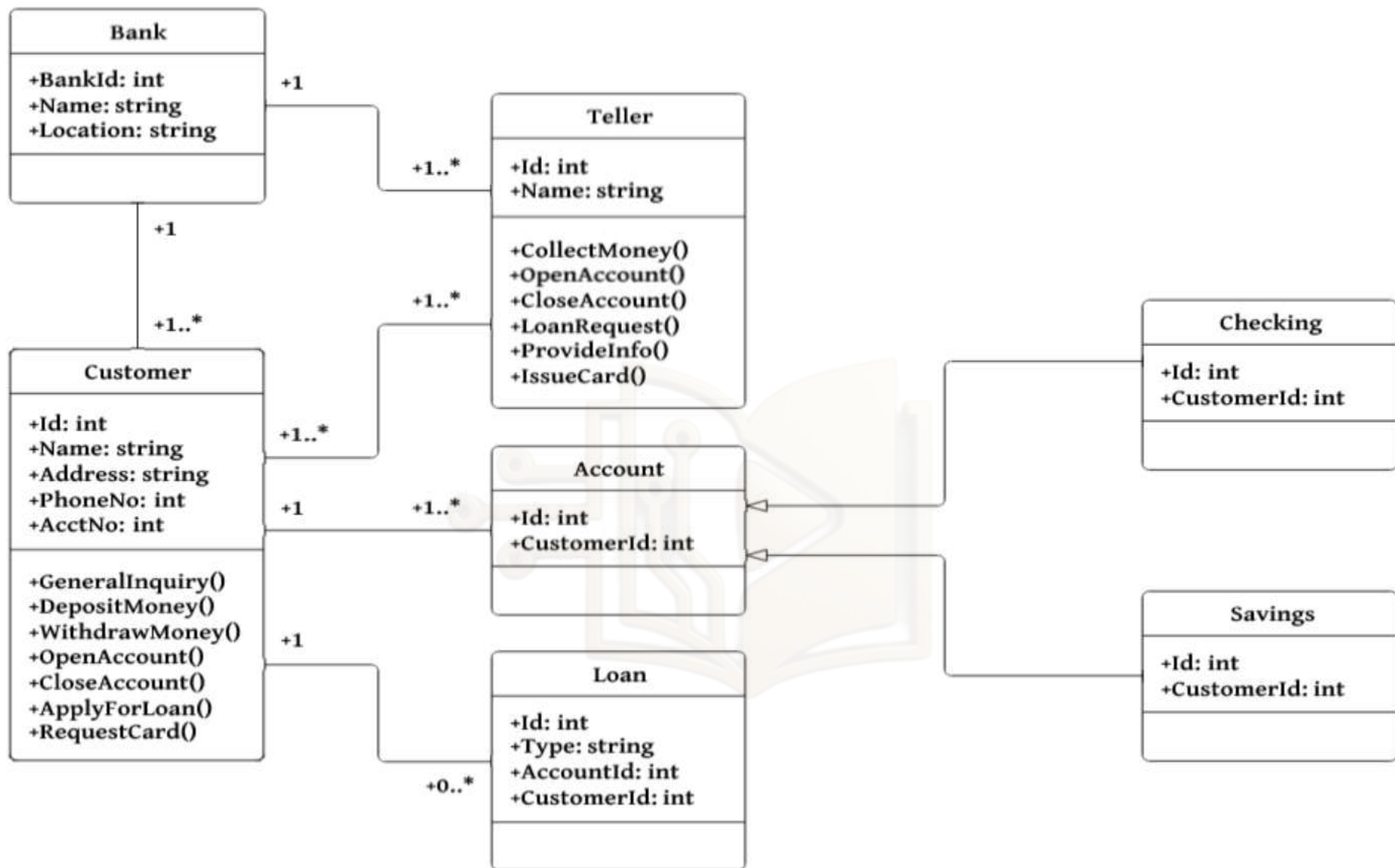
Figure: Class Diagram for Banking System
