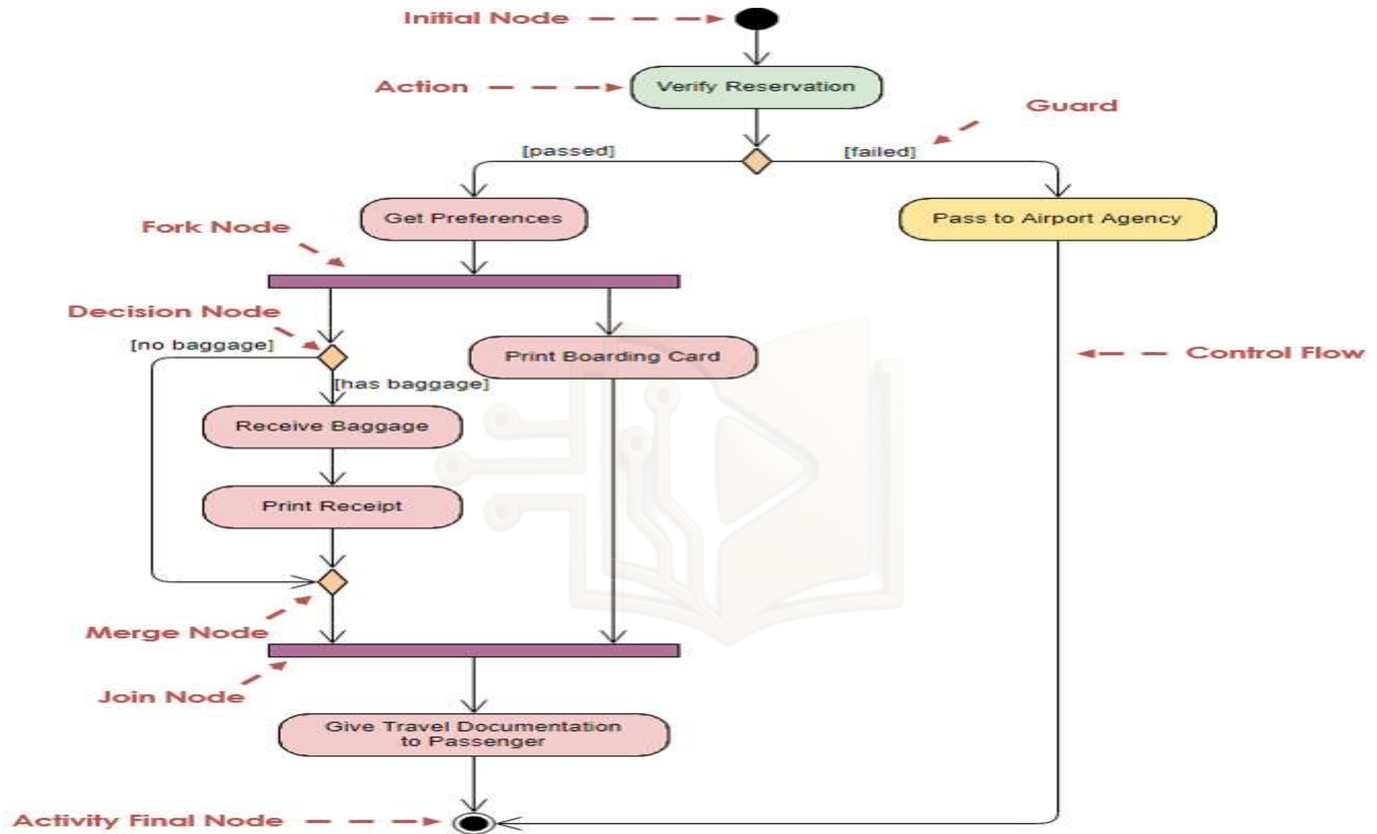
Figure: Activity Diagram Example (Without Swimlane)
