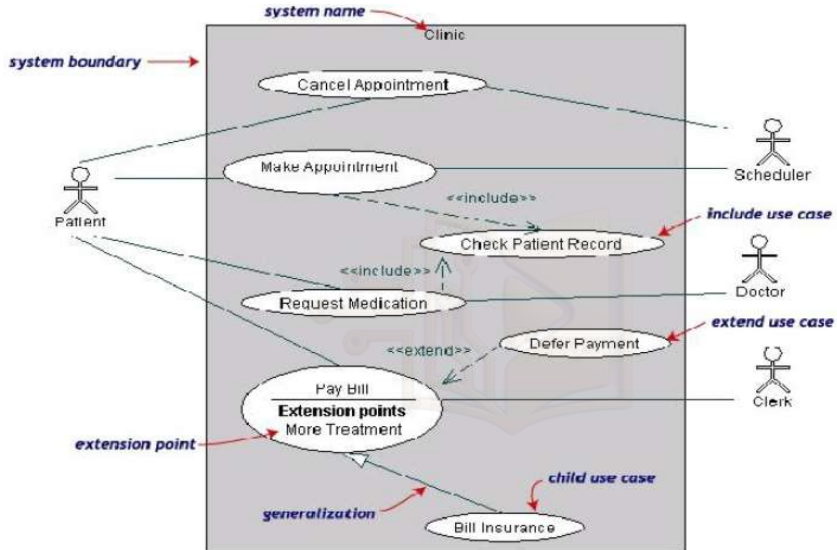
Figure: Use Case Diagram For Clinic System
