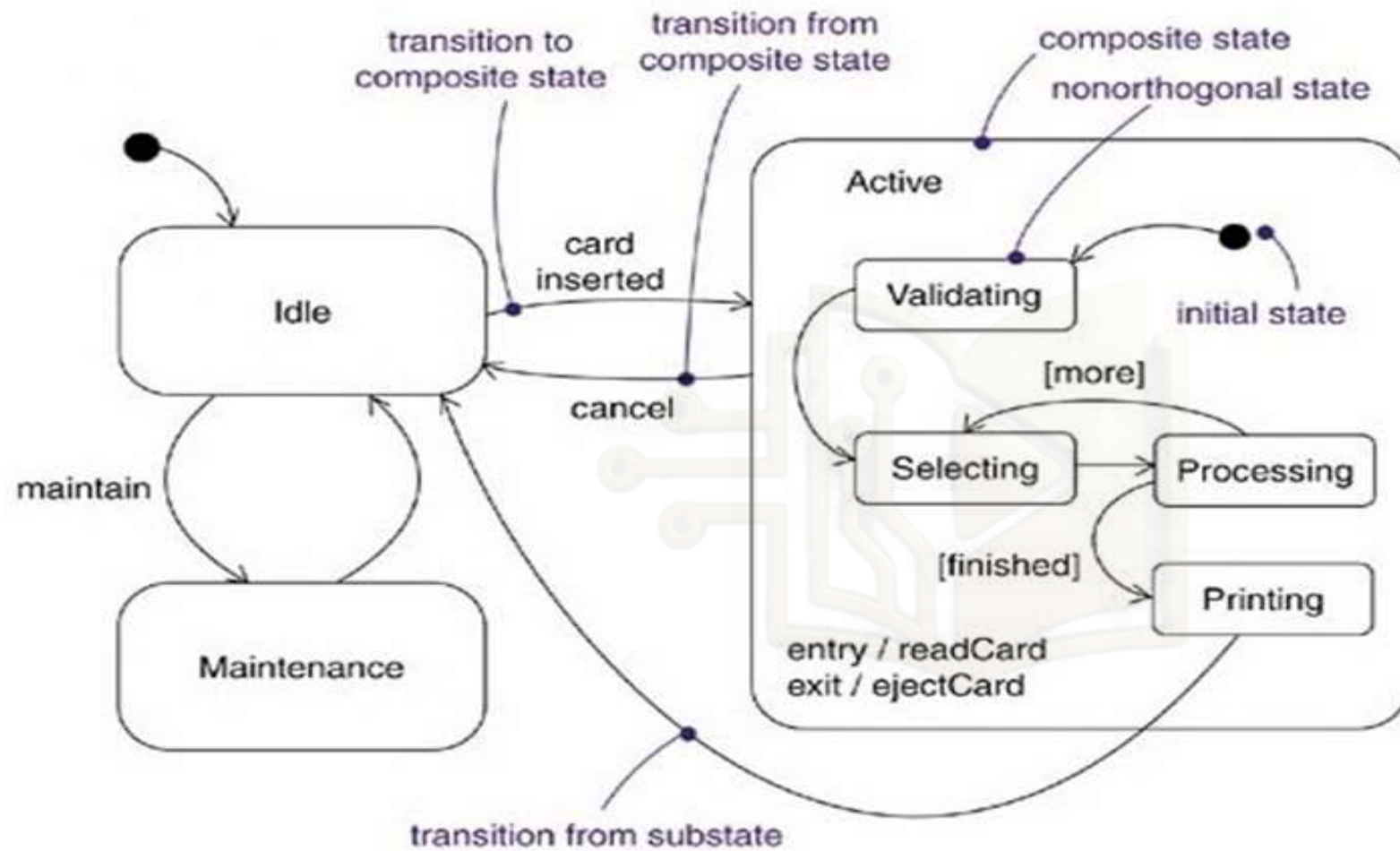
Figure: State Machine Diagram For ATM
