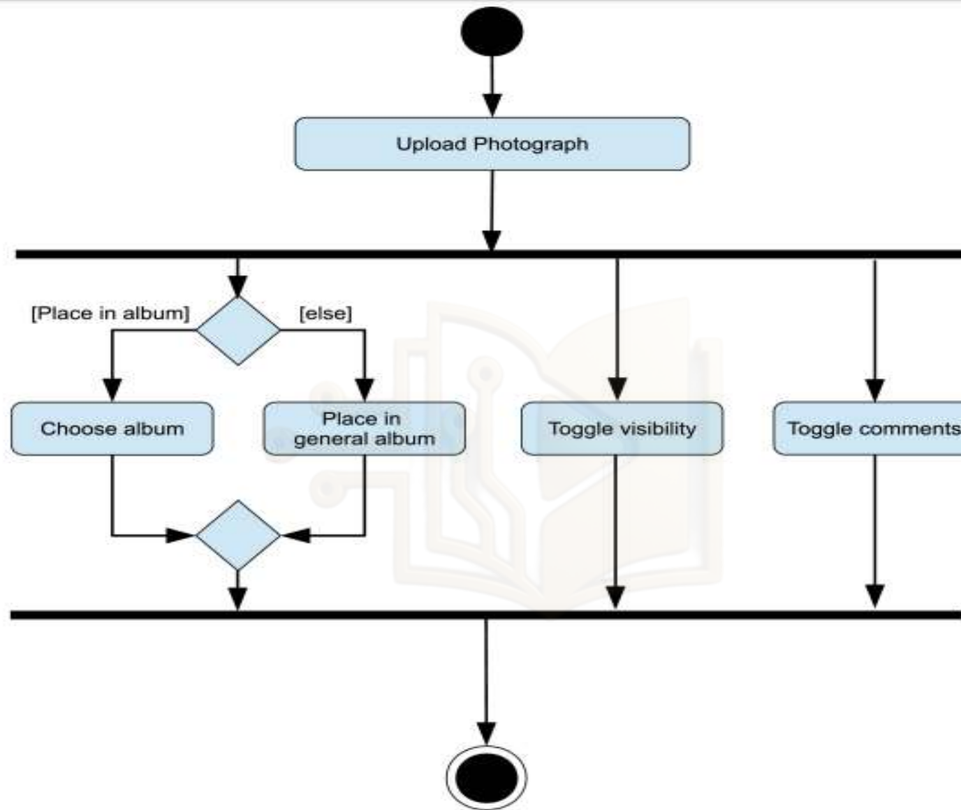
Figure: Activity Diagram Example (Without Swimlane)
