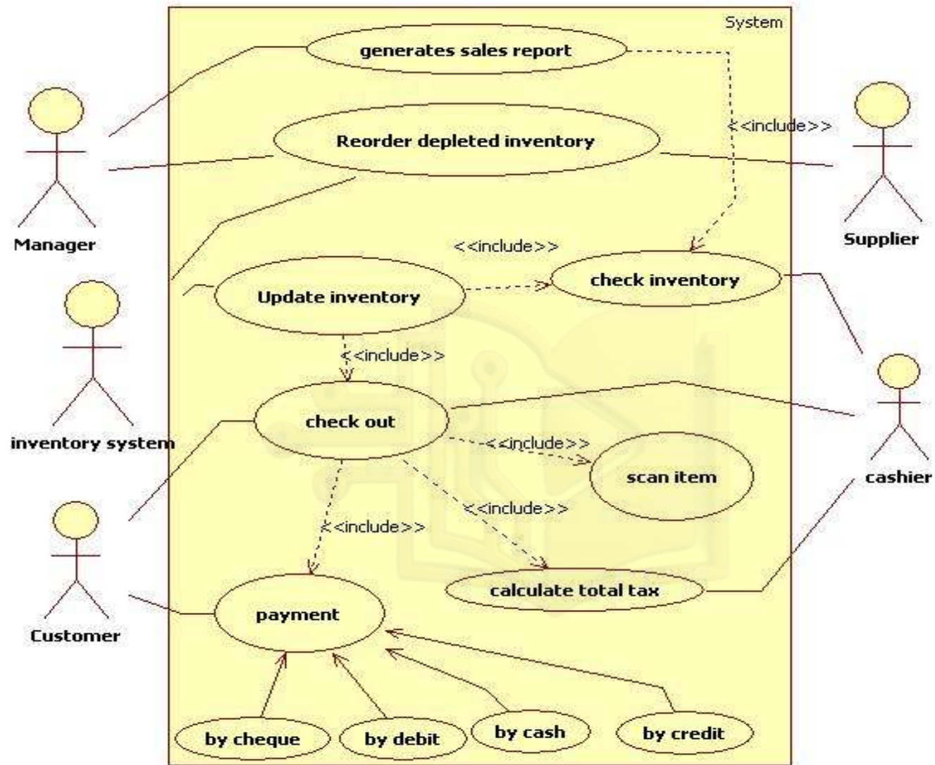
Figure: Use case diagram for POS
