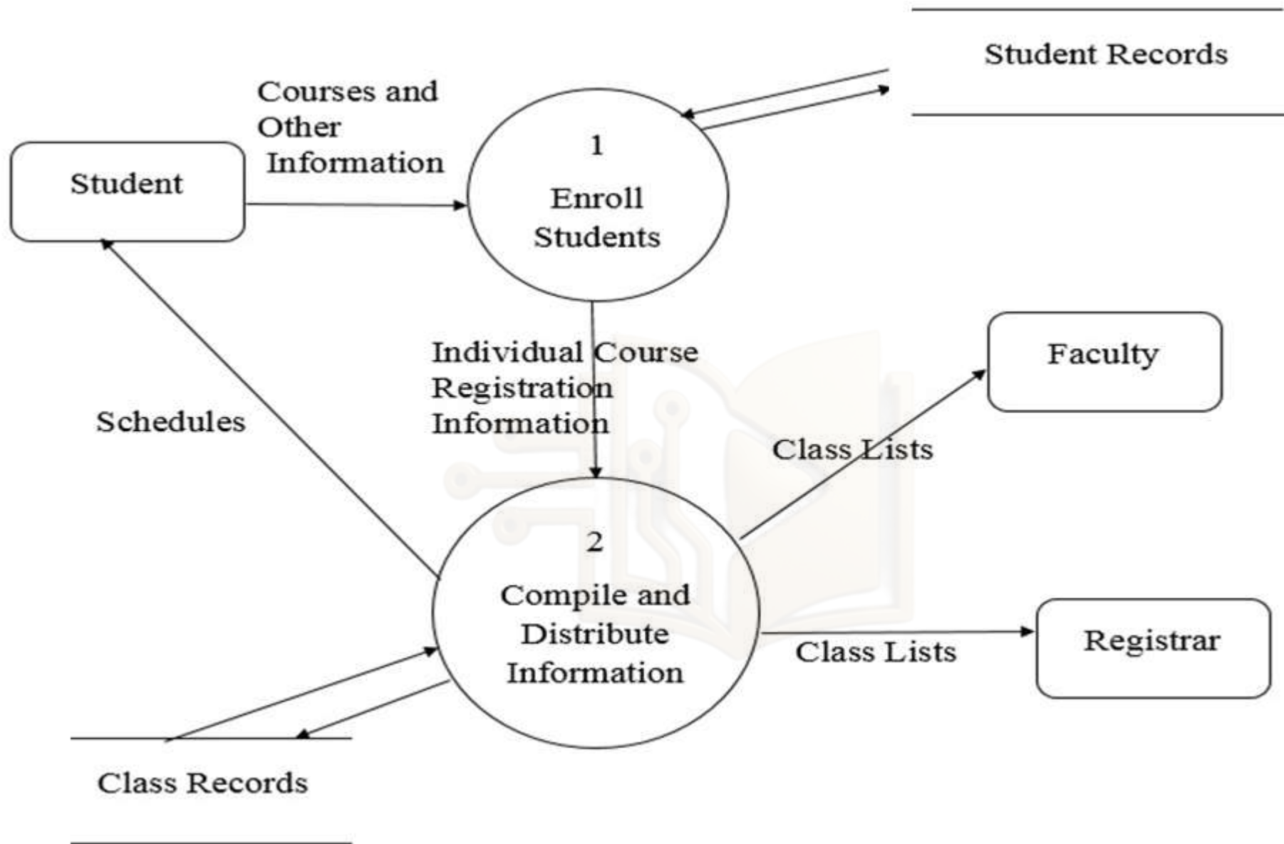
Figure: Level 1 DFD for Course Registration System
