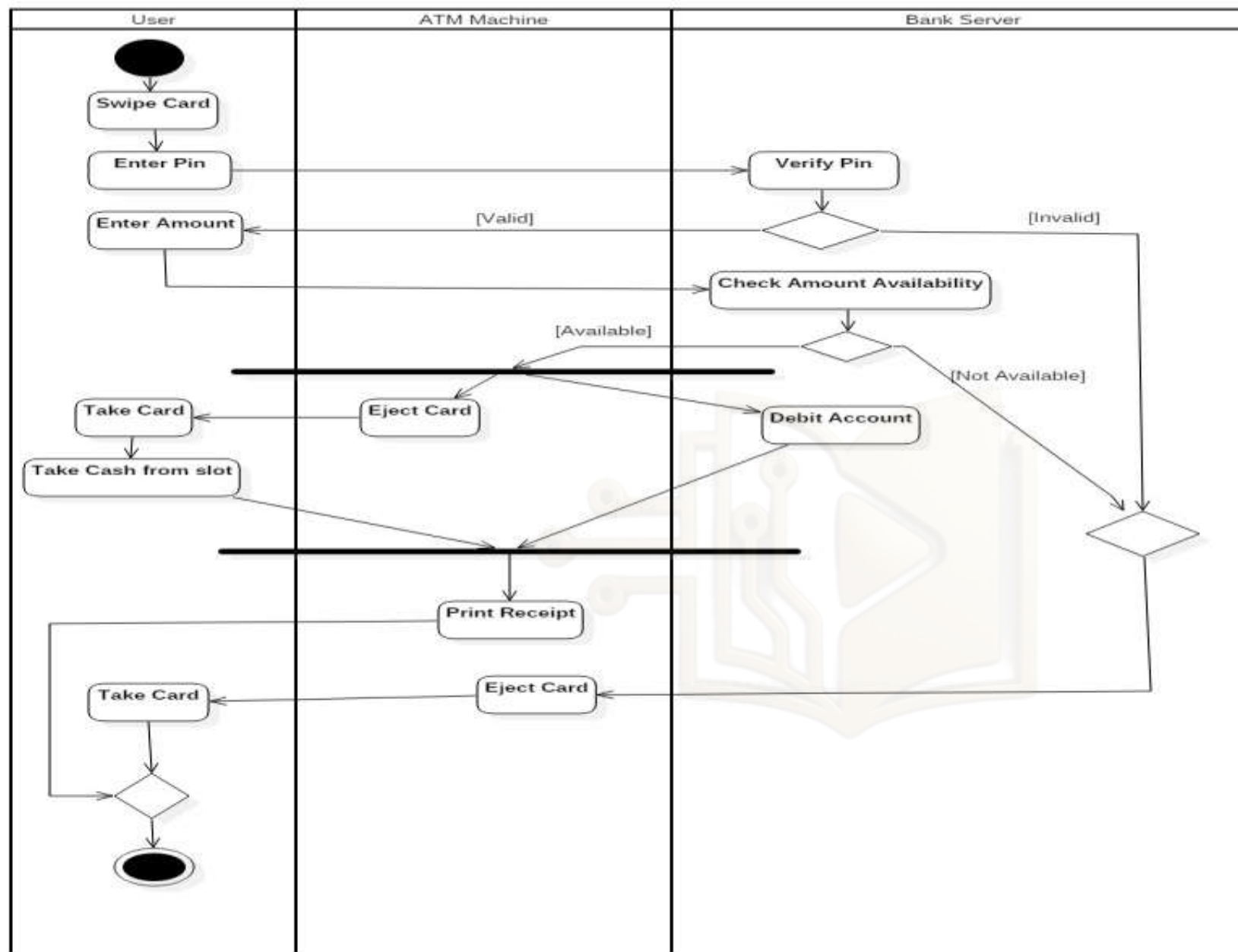
Figure: Activity Diagram of ATM
