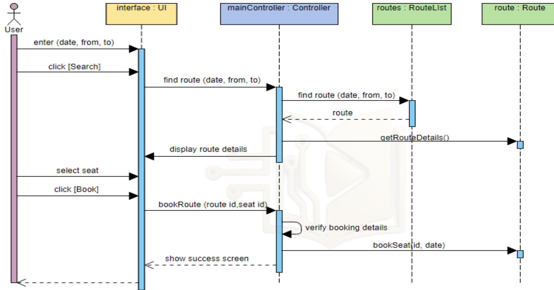
Figure: Online Ticket Booking System
